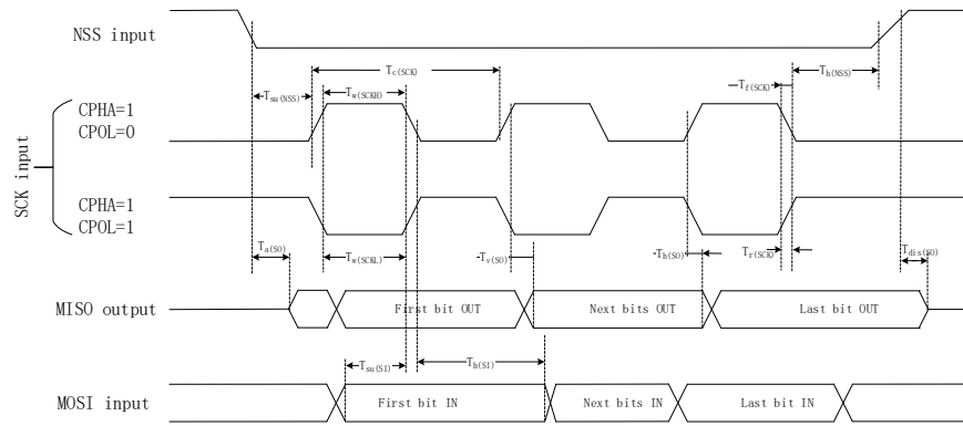
Figure 5-4 SPI timing diagram – Slave Mode and CPHA=1
