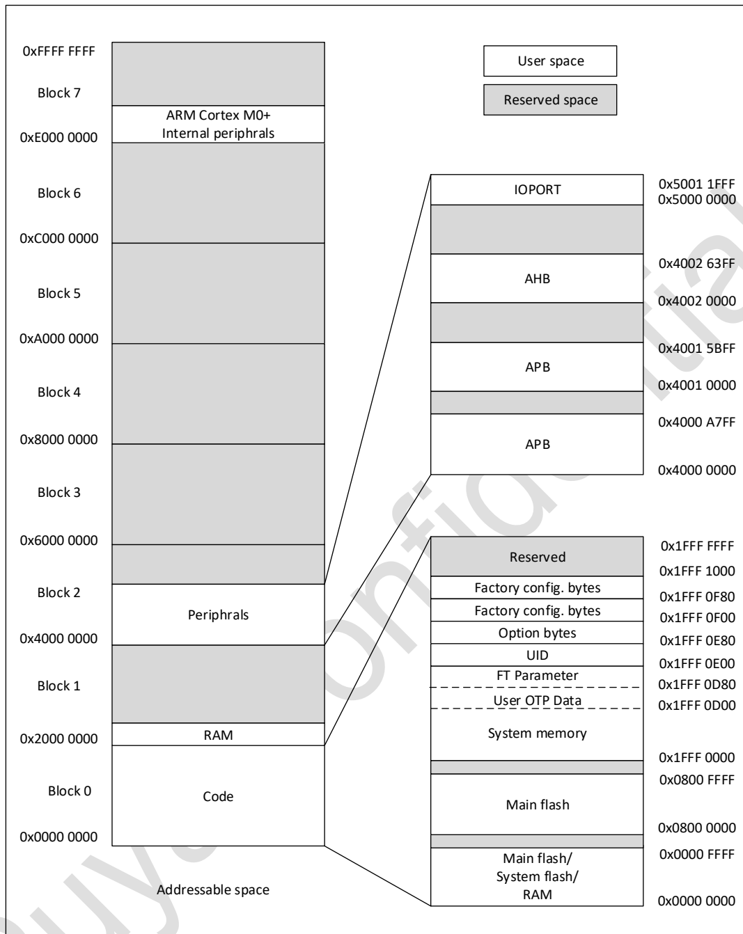
Figure 4-1 Memory mapping
