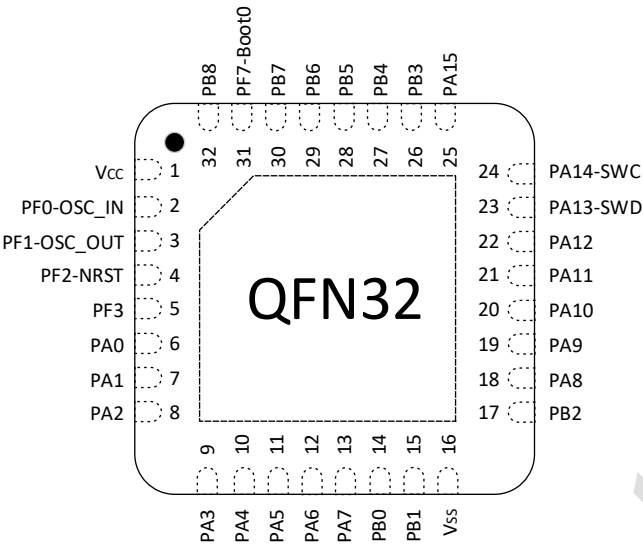
Figure 3-7 QFN32(4*4) Pinout2 PY32F031K2xU7 (Top view)
