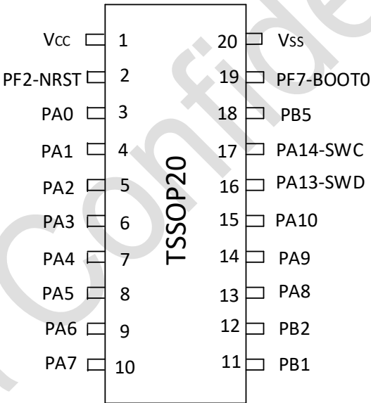
Figure 3-8 TSSOP20 Pinout1 PY32F031F1xP6 (Top view)
